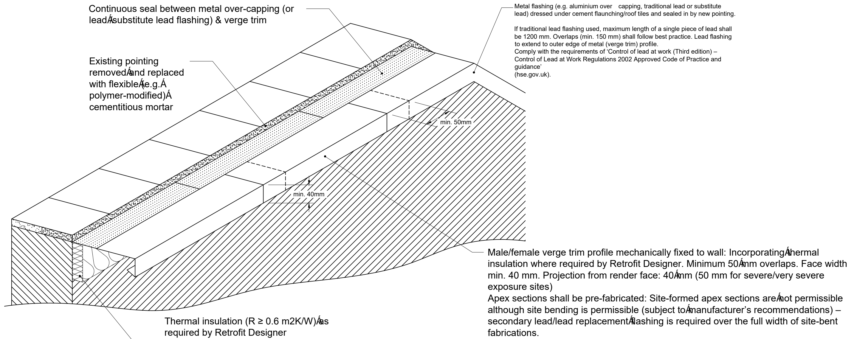
Title : VERGE APEX - IMPROVED ROOFLINE CLOSURE - PRE-FORMED APEX
